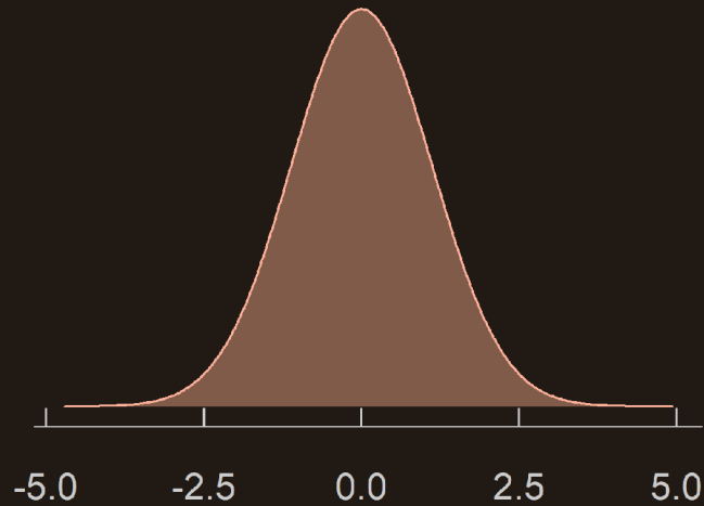
Normal distribution
