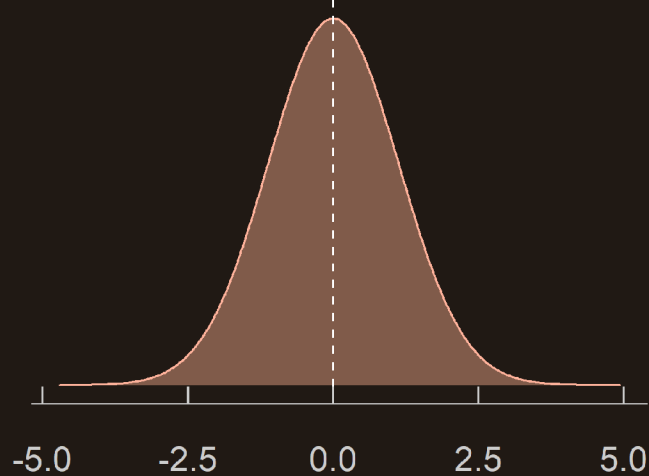
Normal distribution
