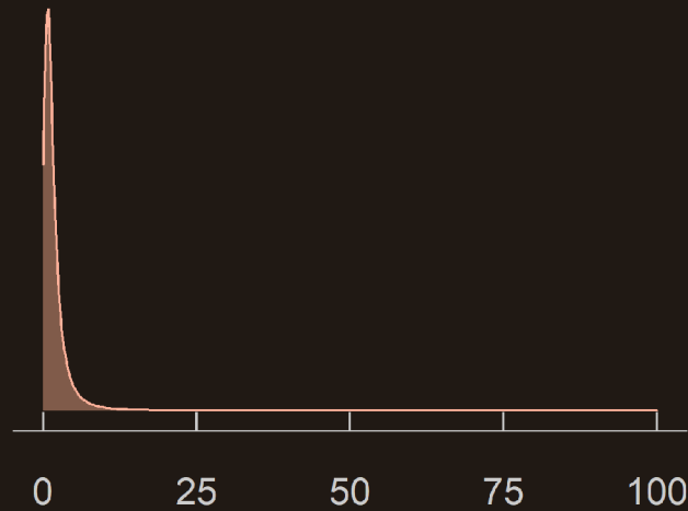
Log-normal distribution
