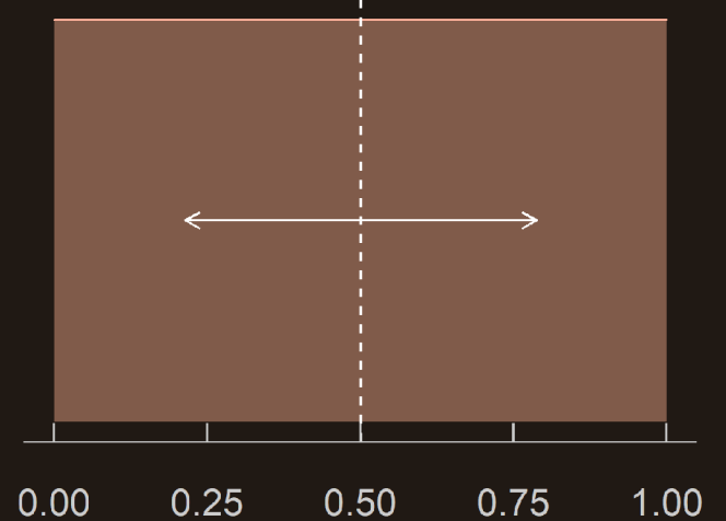
Uniform distribution
