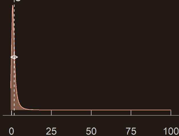
Log-normal distribution
