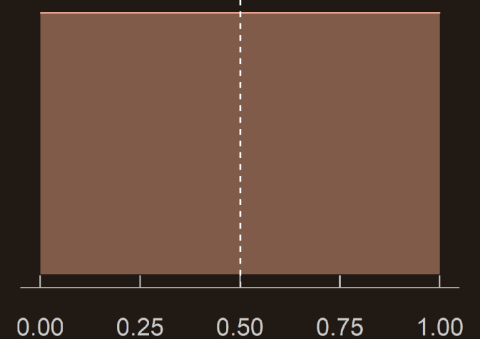
Uniform distribution
